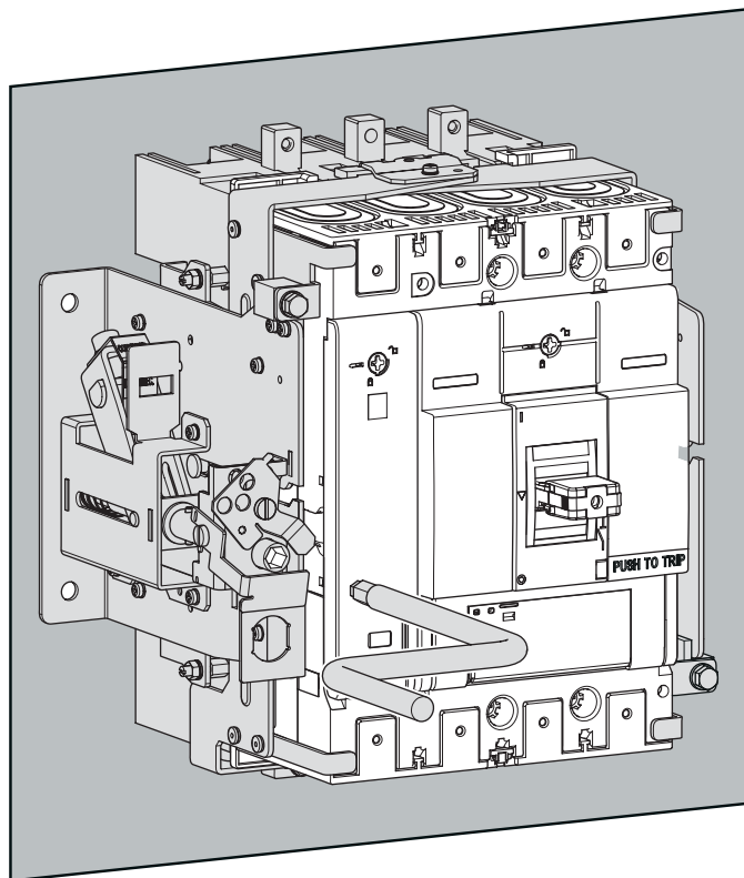
x630 withdrawable
