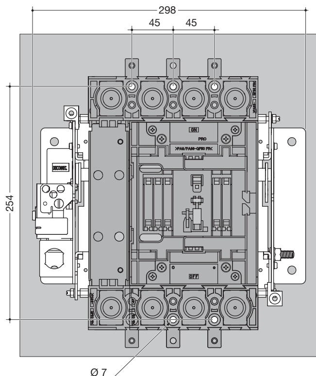
Drilling drawing Withdrawable back plate x630 3P + 4P
