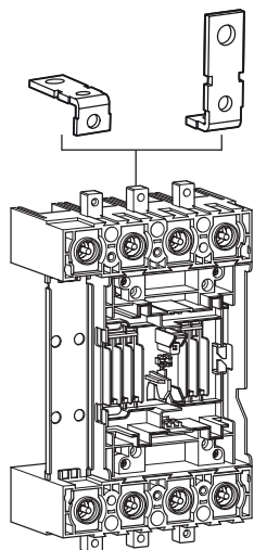
Plug-in base
