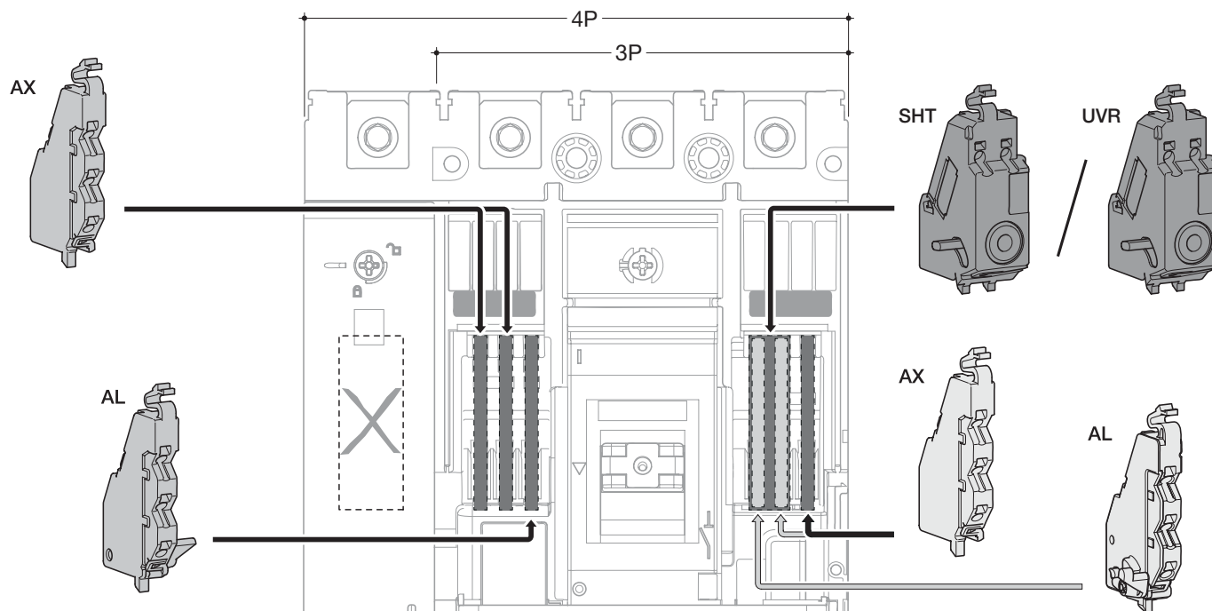
Auxiliary location
