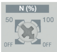
Neutral protection dial LSnI trip unit
