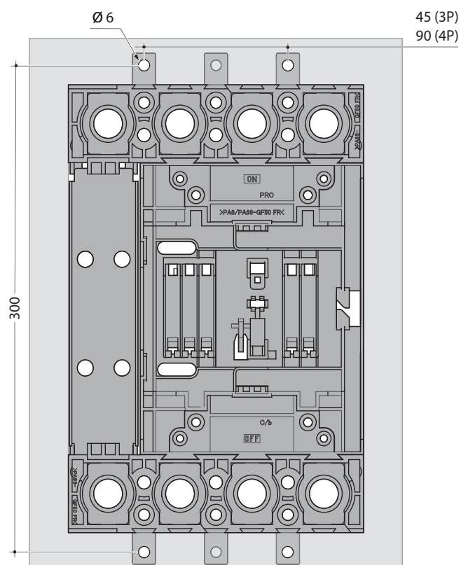
x630 plug-in kit drilling pattern for flush mounting
