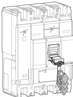
Padlocking kit
