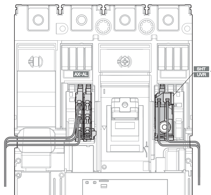
Auxiliary cabling
